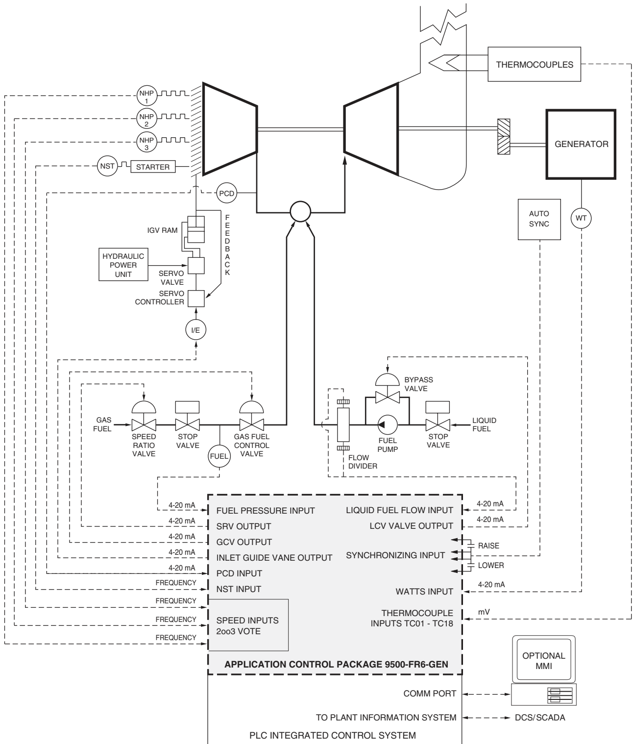
Simplified schematic showing a Petrotech GE Frame 6® gas turbine generator drive application control package integrated into an advanced PLC-based control system. Shown with dual fuel system.
